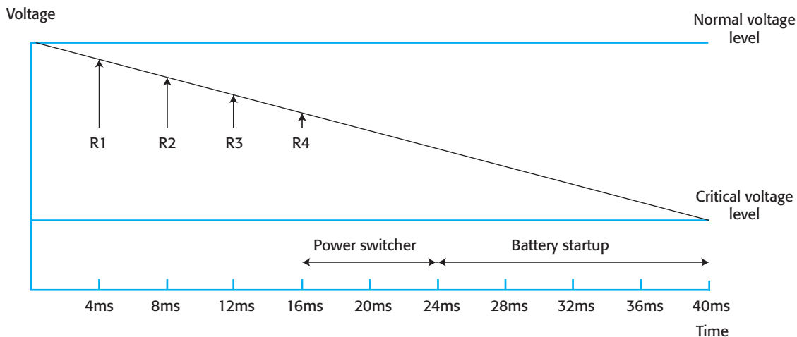
Figure 21.15 Power failure timing analysis
